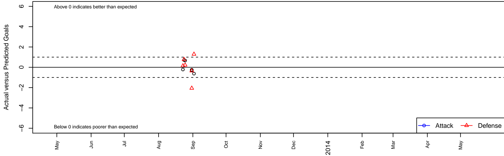
Montesano Renegades G99 Dots are actual minus expected GF (blue circles) and GA (red triangles). Blue line is smoothed change in attack strength. Red is smoothed change in defense strength.
